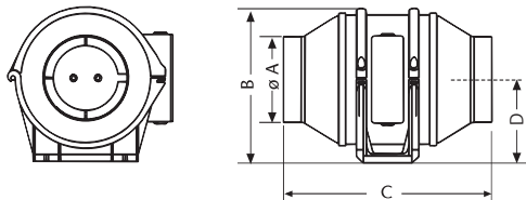
DUCT IN-LINE 150-200
